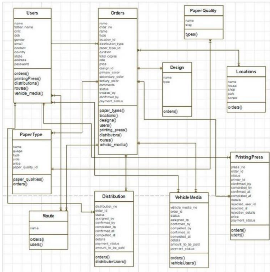
Figure 4.2: Class Diagram
