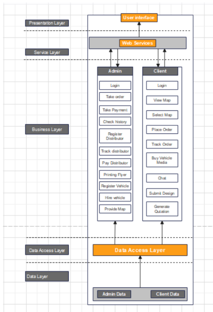
Figure 4.1: Architecture Diagram
